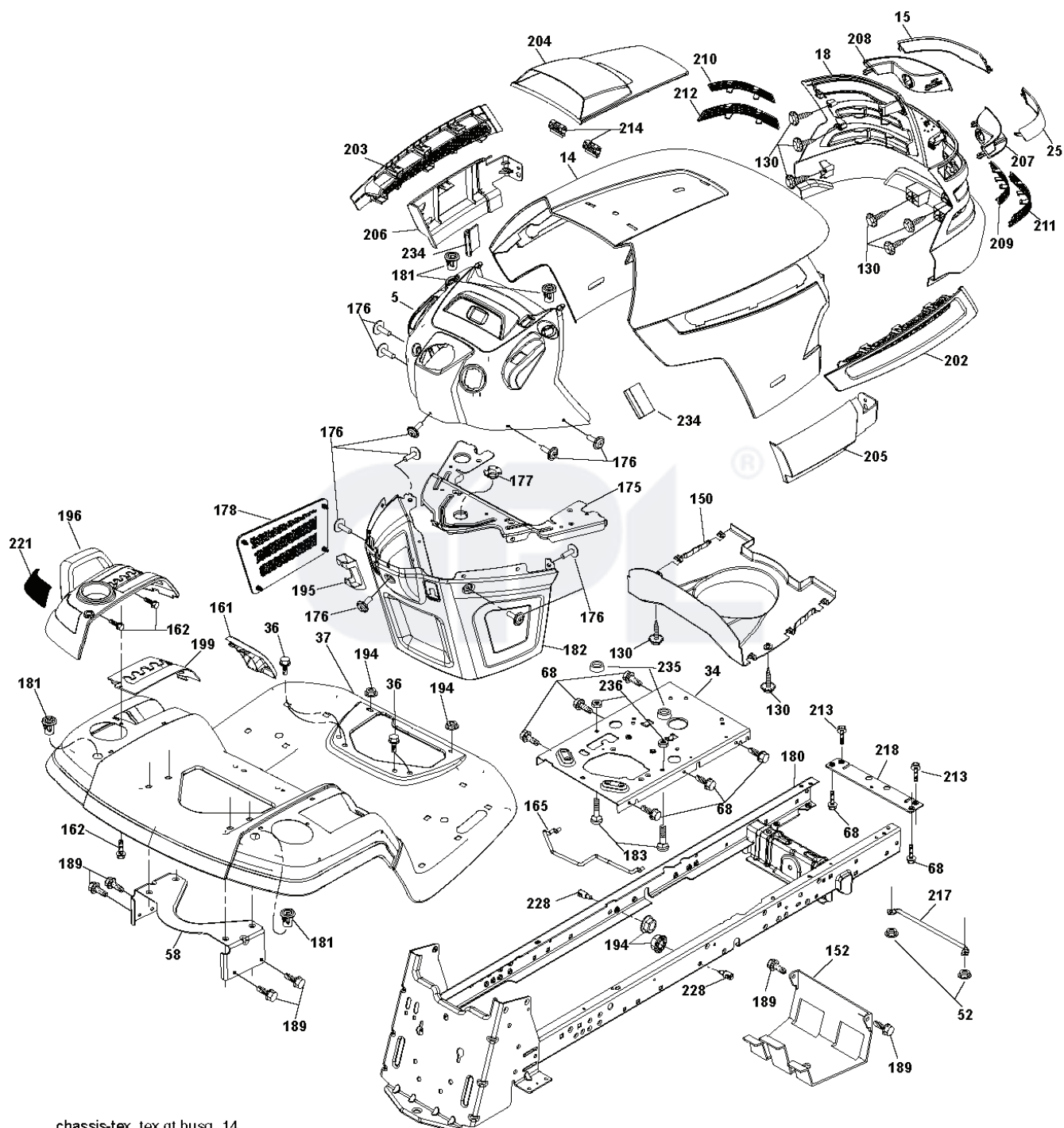
chassis-tex_tex gt husq_14
