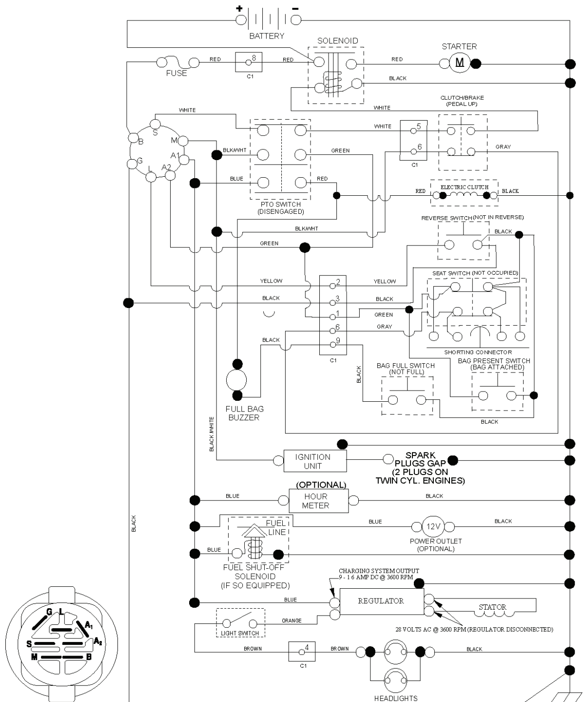
IGNITION SWITCH
