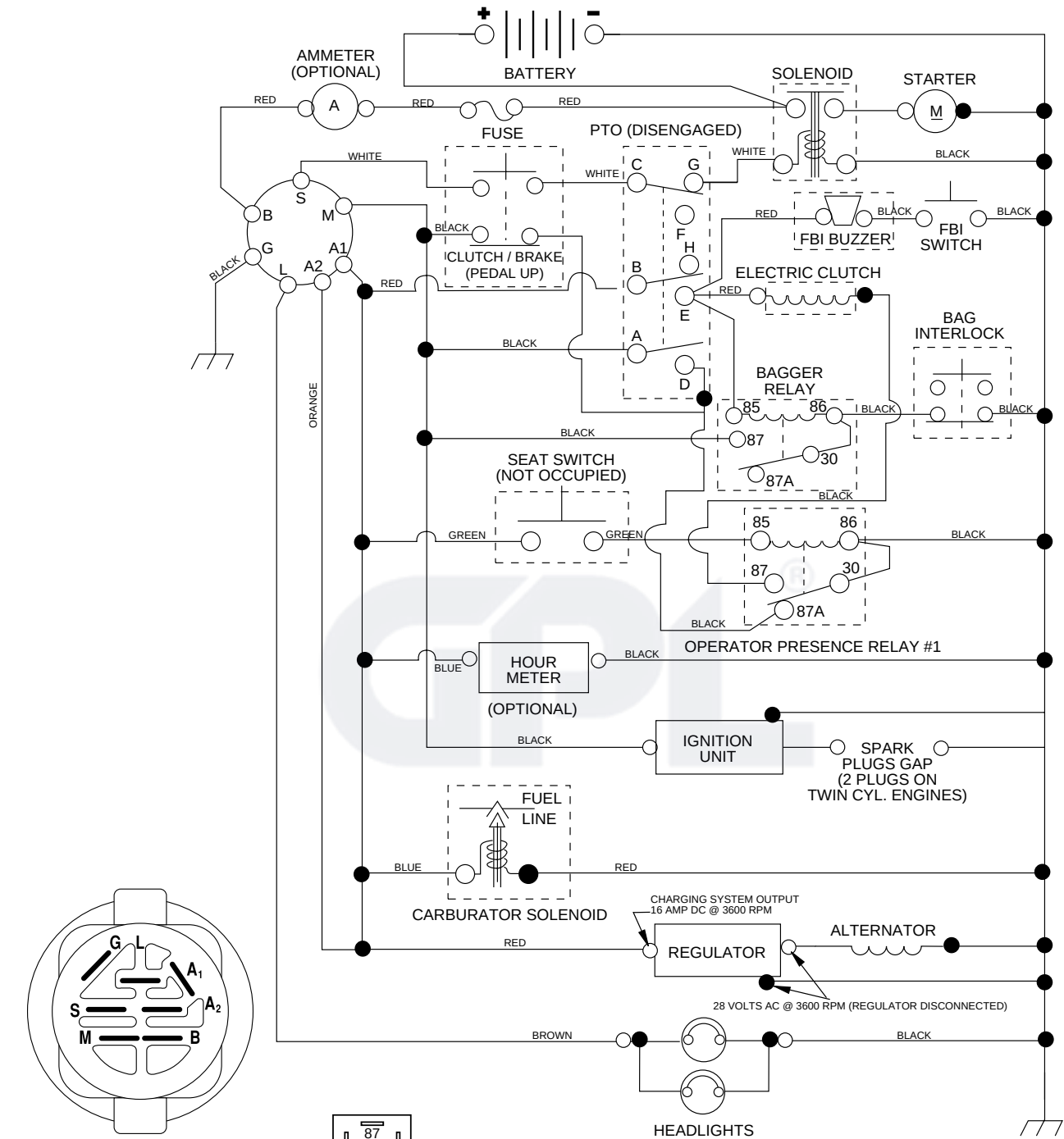
IGNITION SWITCH
