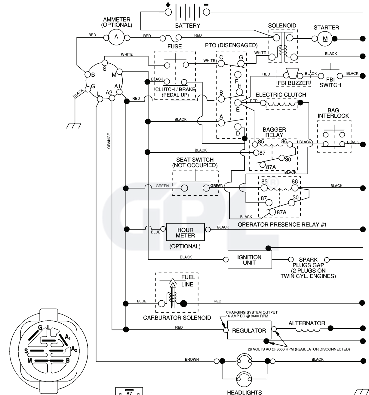
IGNITION SWITCH
