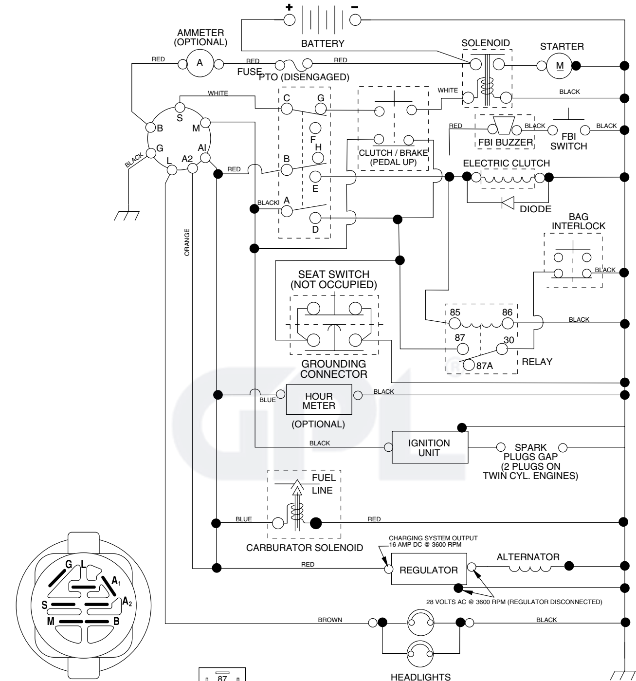
IGNITION SWITCH
