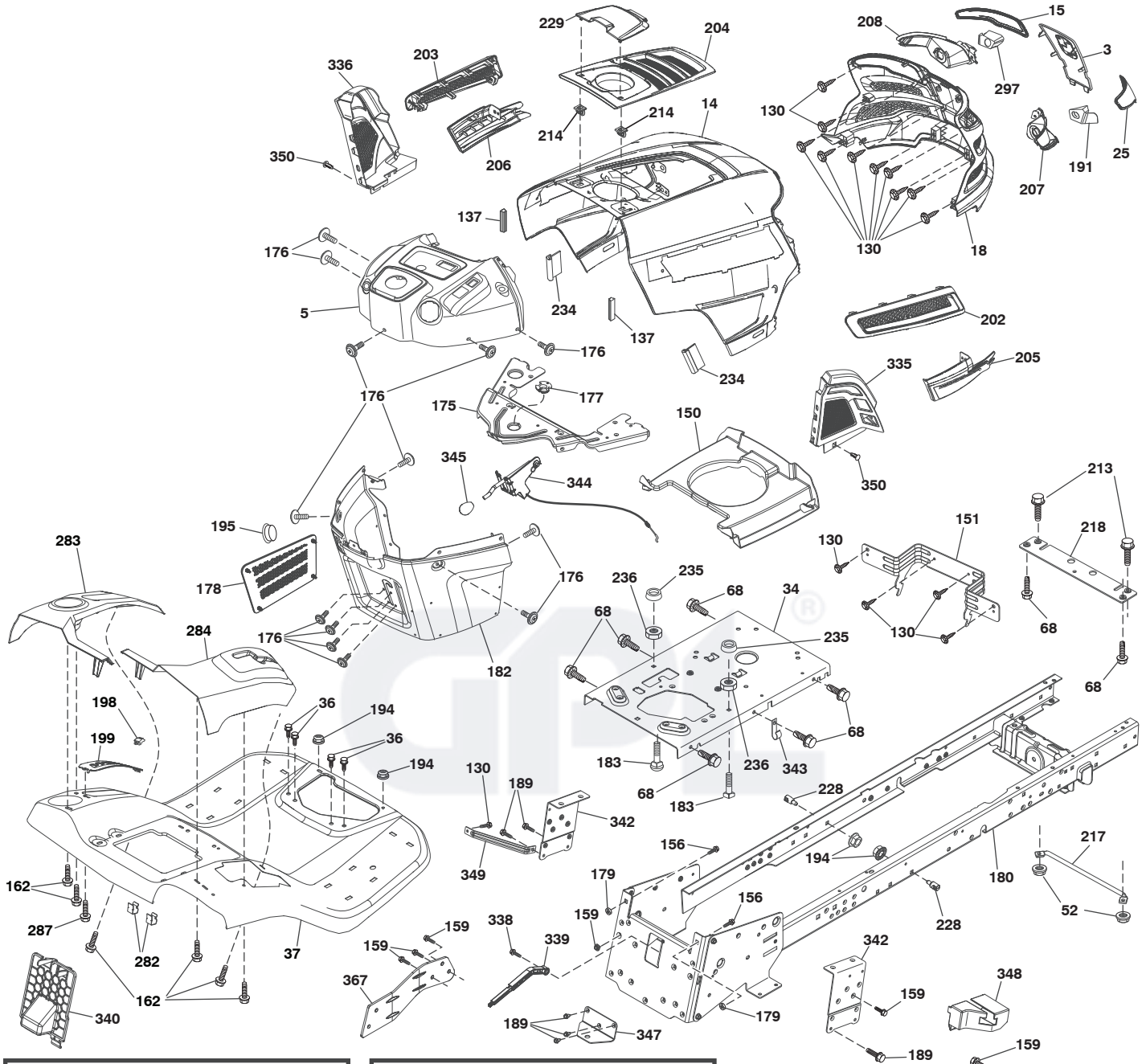
TUBE-SUPPORT BAGGER MODELS ONLY
