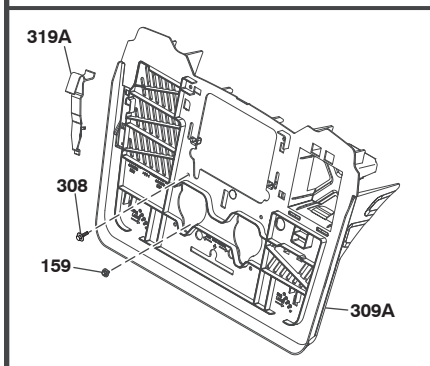
TUBE-SUPPORT BAGGER MODELS ONLY
