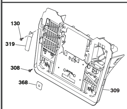
BRACKET-SUPPORT BAGGER MODELS ONLY
