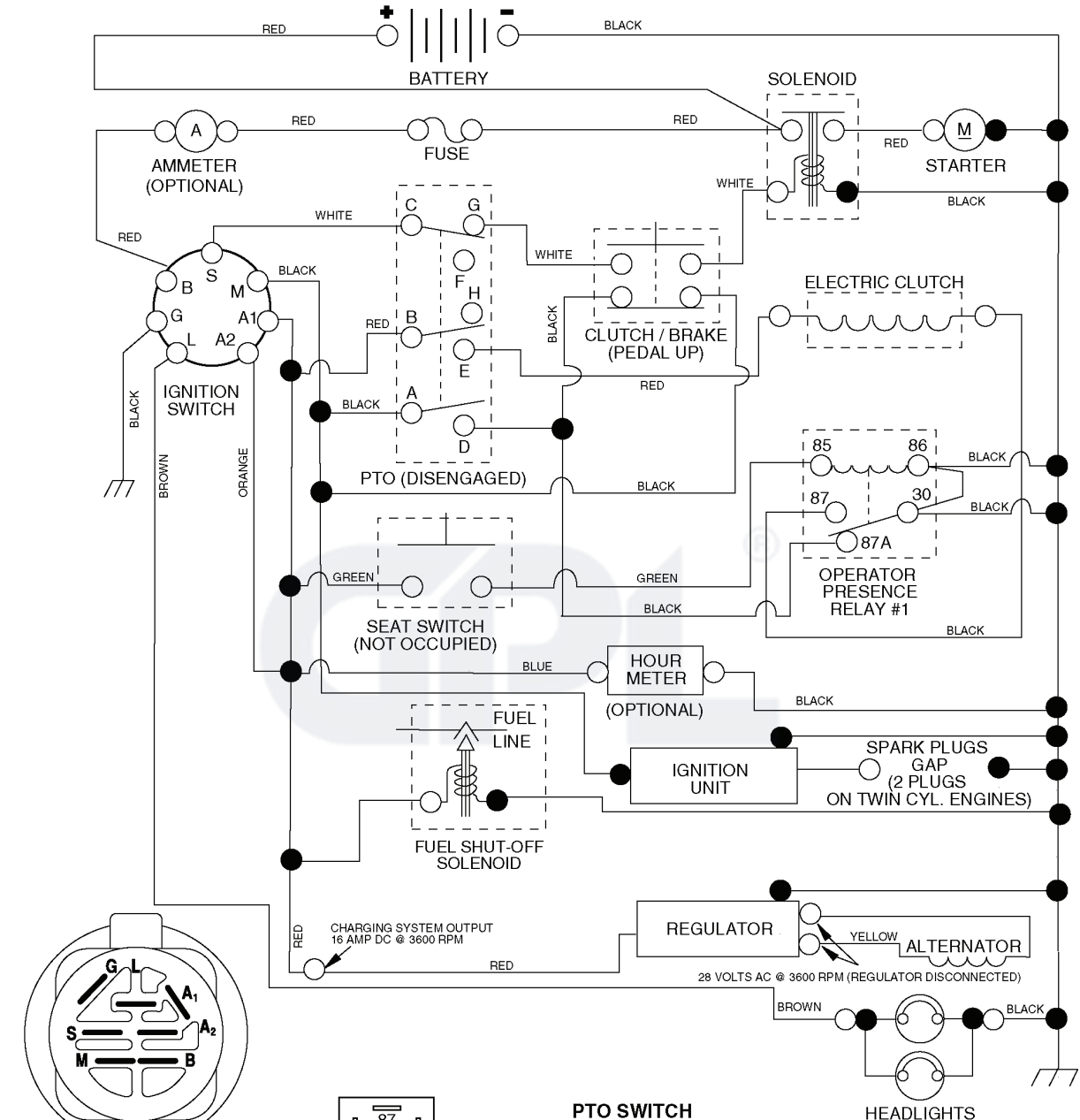
IGNITION SWITCH
