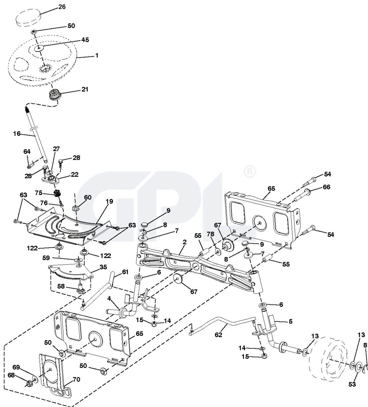
Steering-tex_LEGND2_58
