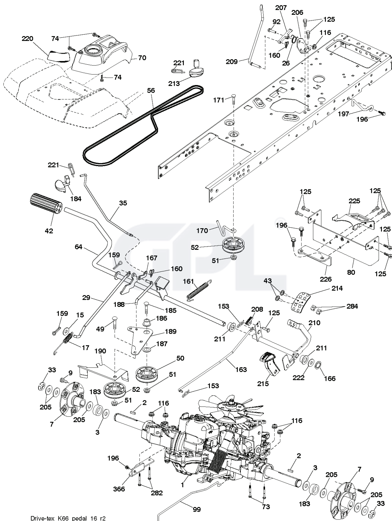
Drive-tex_K66_pedal_16_r2
