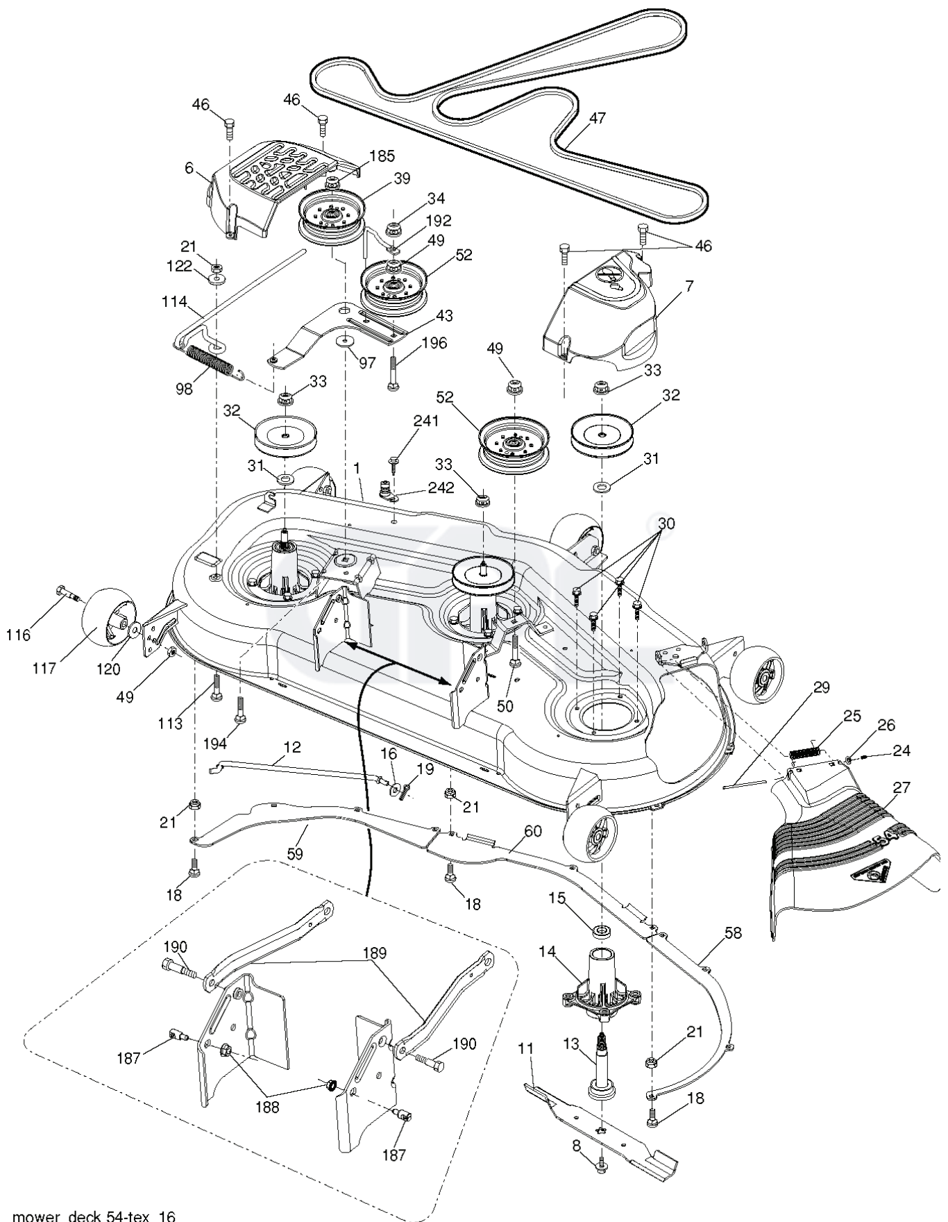
mower_deck 54-tex_16
