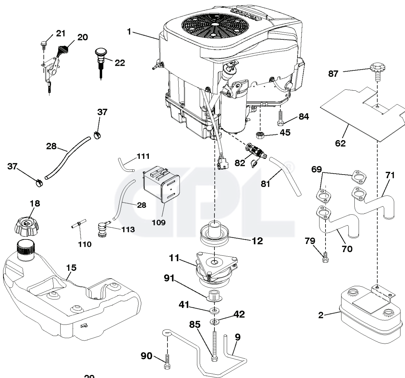
SPARK ARRESTER KIT
