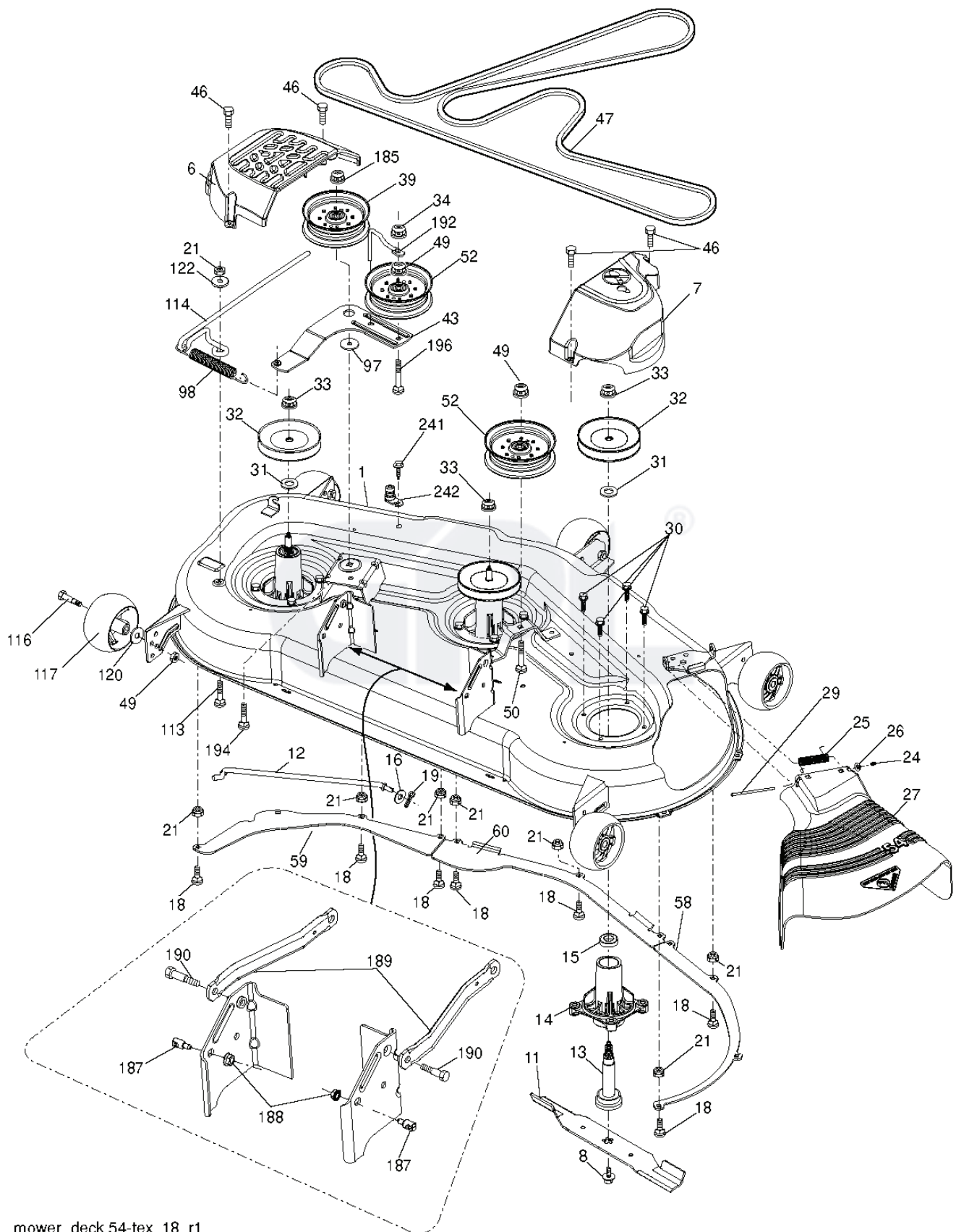
mower_deck 54-tex_18_r1
