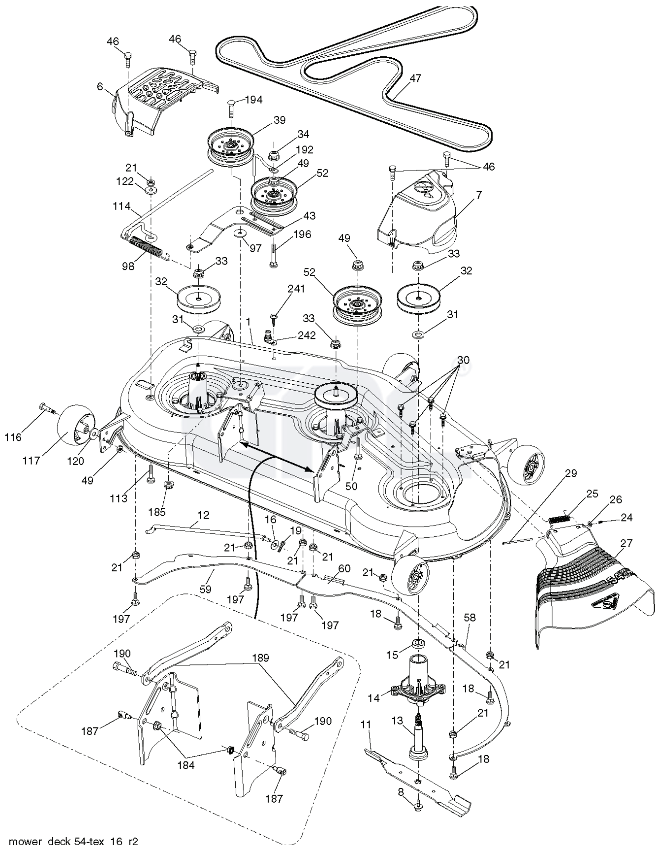
mower_deck 54-tex_16_r2
