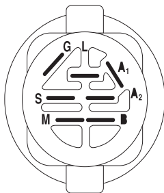
IGNITION SWITCH
