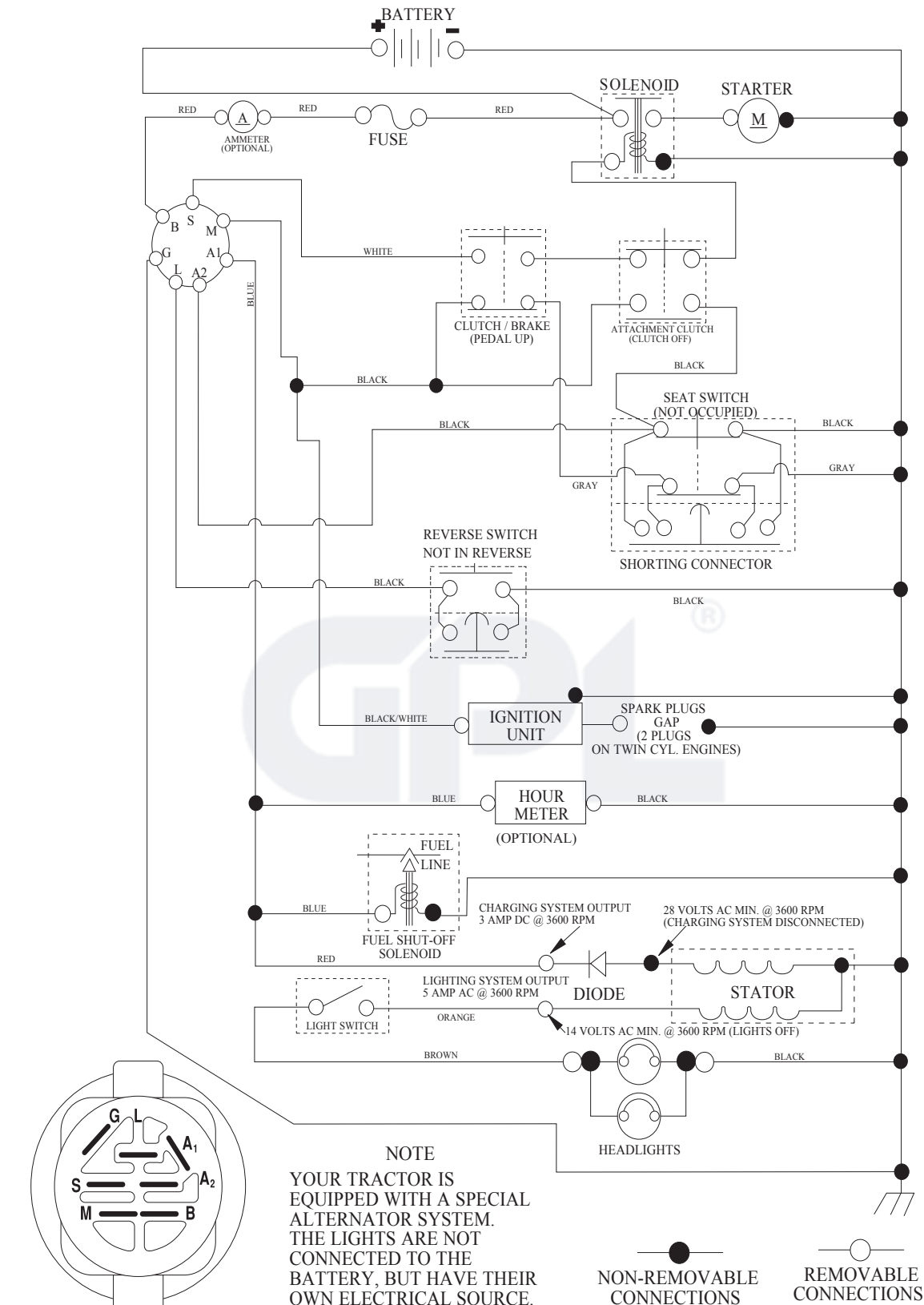
IGNITION SWITCH
