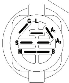
IGNITION SWITCH
