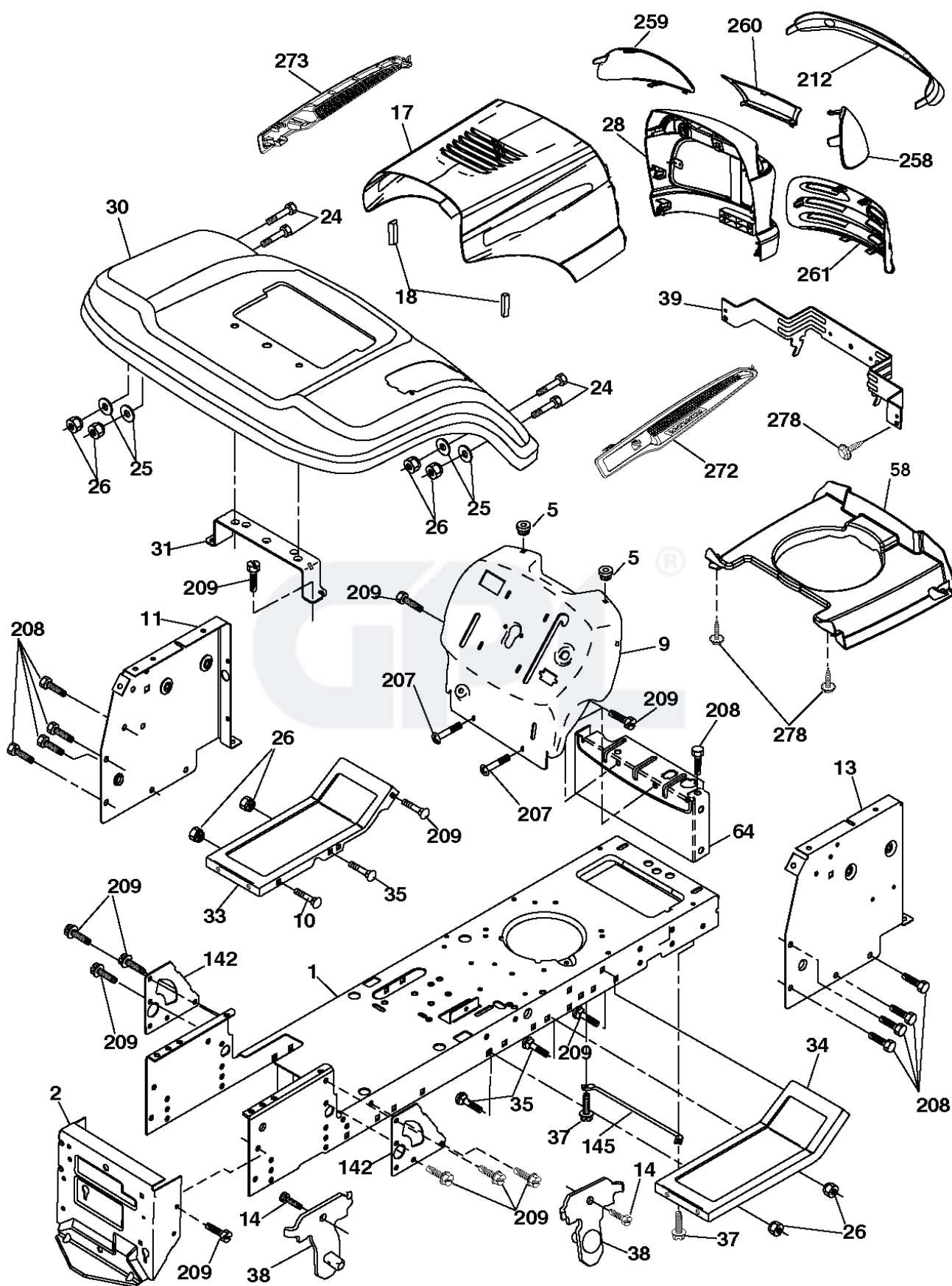
chassis-STL_Husq Laser-SV_1_r3
