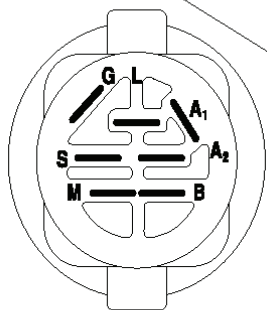
IGNITION SWITCH
