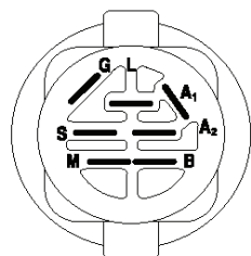
POSITION CIRCUIT "MAKE" OFF M+G+A1 RUN/OVERRIDE B+A1 RUN B+A1 L+A2 START B + S + A1
