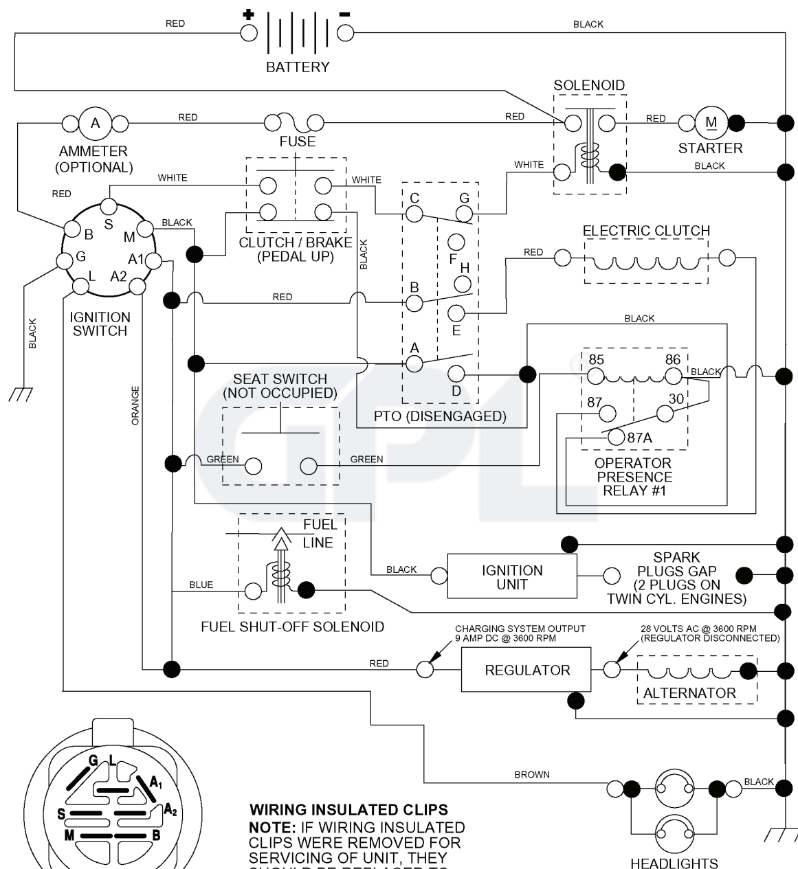
IGNITION SWITCH
