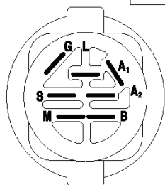
IGNITION SWITCH
