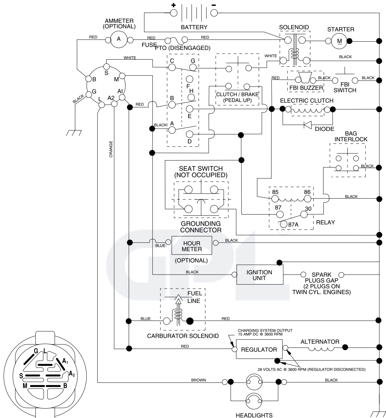
IGNITION SWITCH
