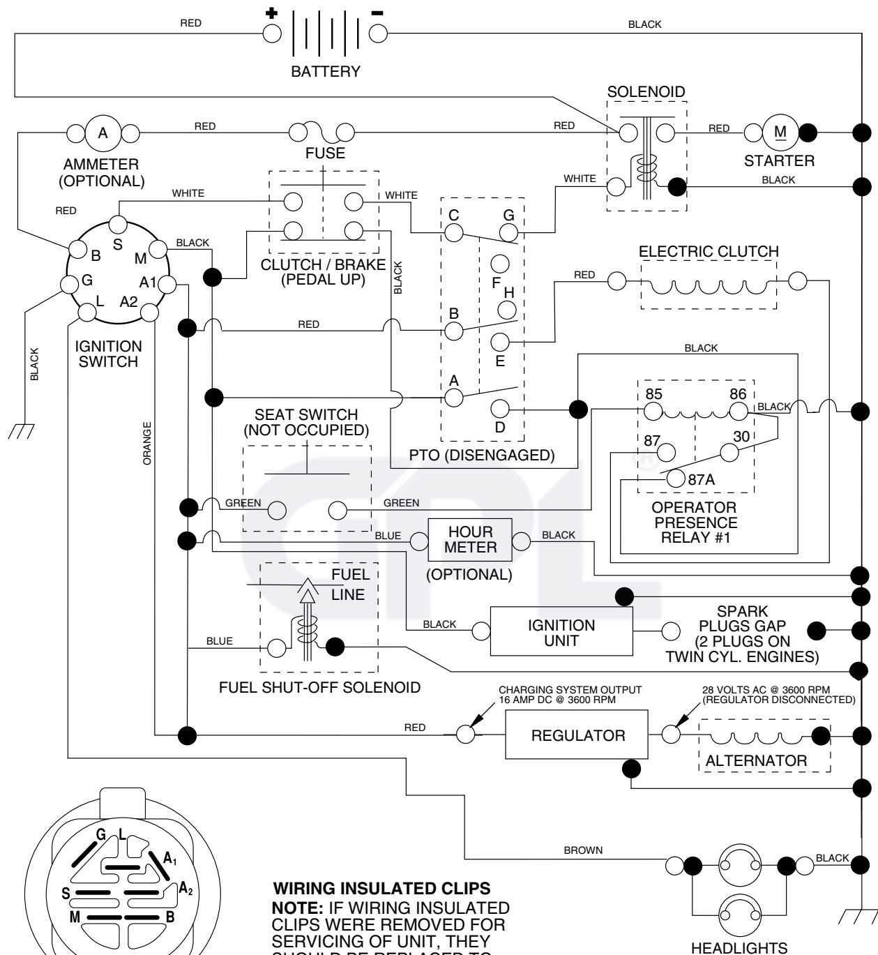
IGNITION SWITCH
