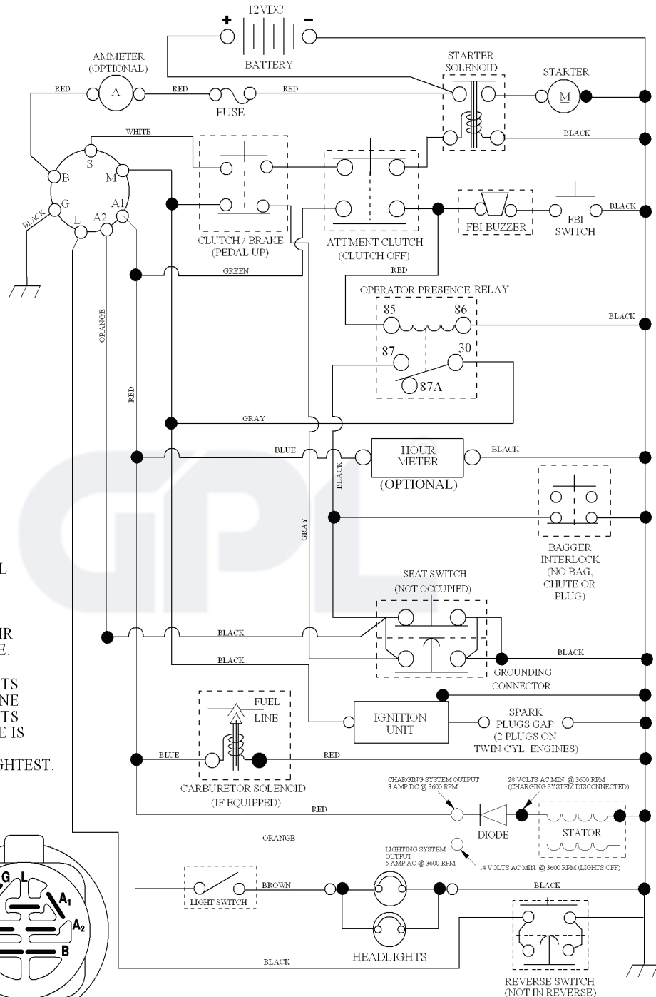
IGNITION SWITCH
