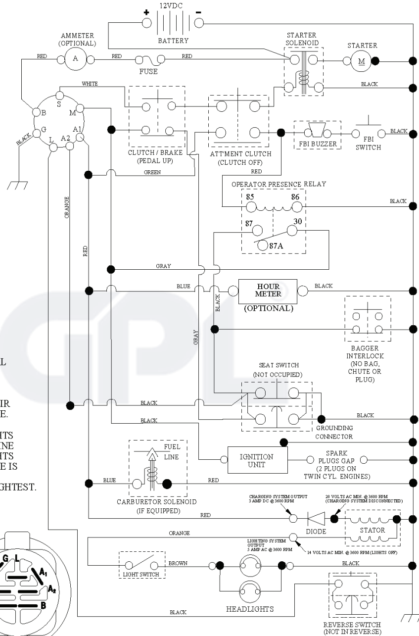
IGNITION SWITCH
