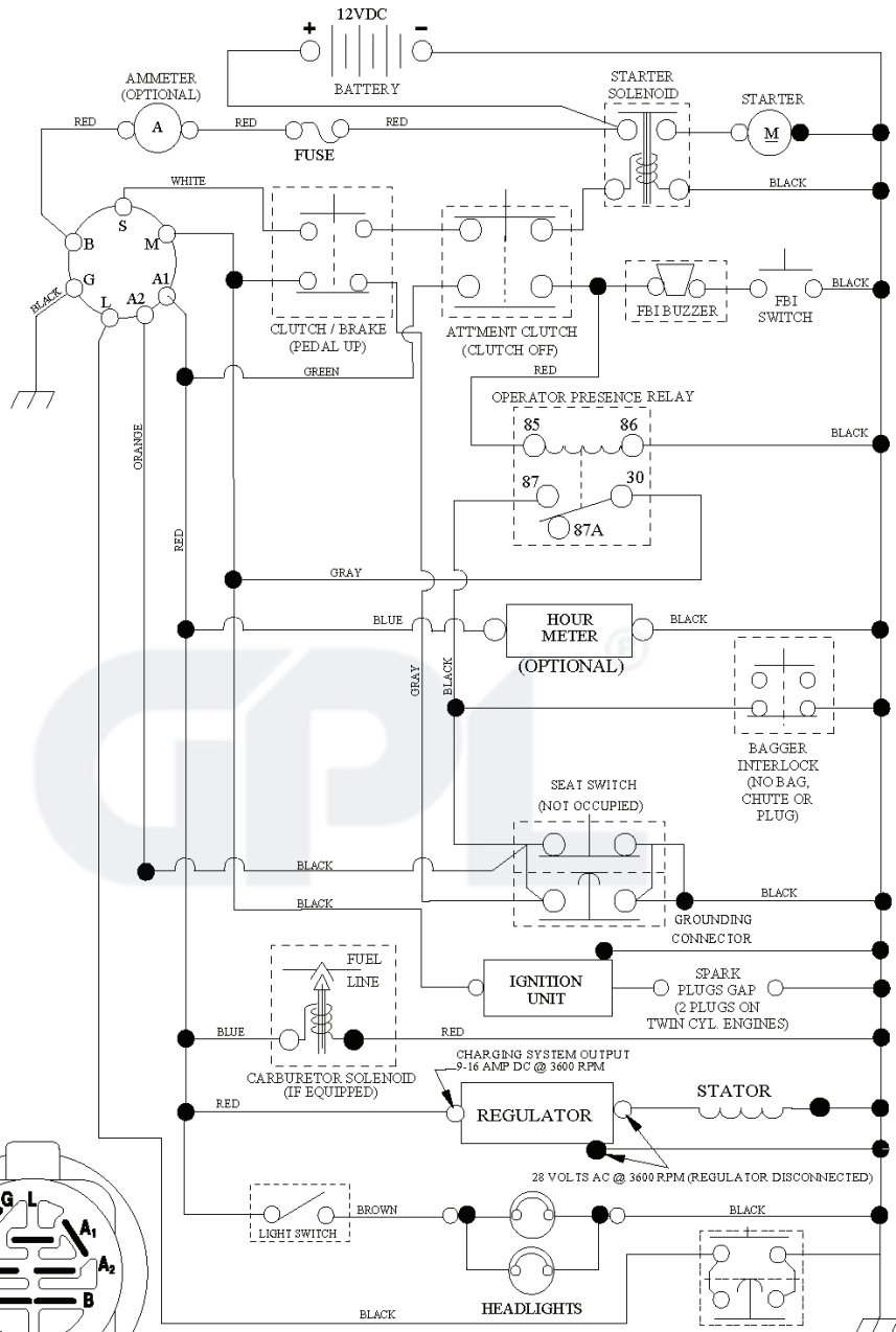
IGNITION SWITCH
