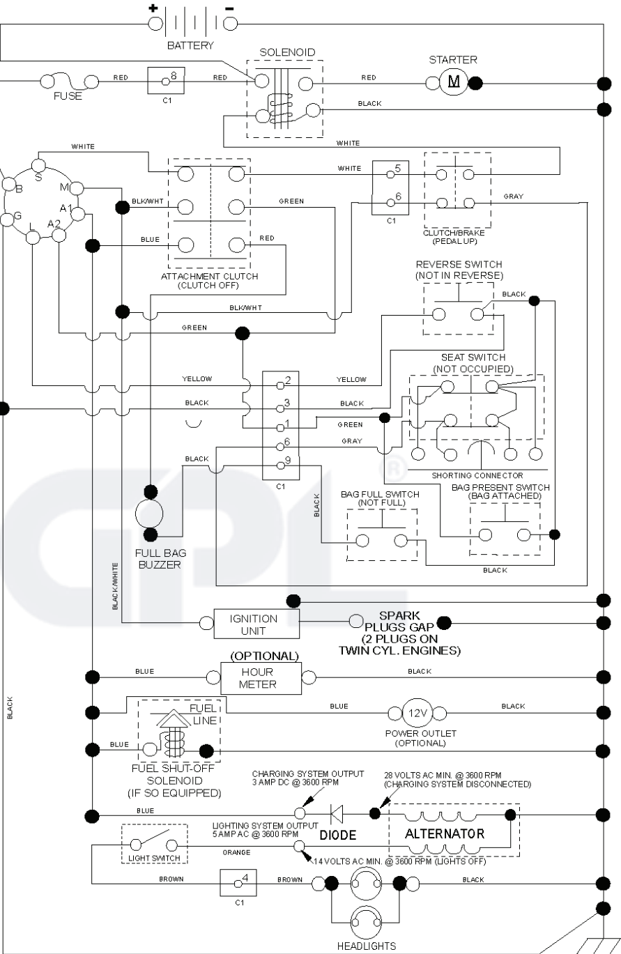
NON-REMOVABLE CONNECTIONS
