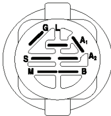
IGNITION SWITCH
