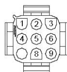
CHASSIS HARNESS CONNECTOR (C1) (MATING SIDE)
