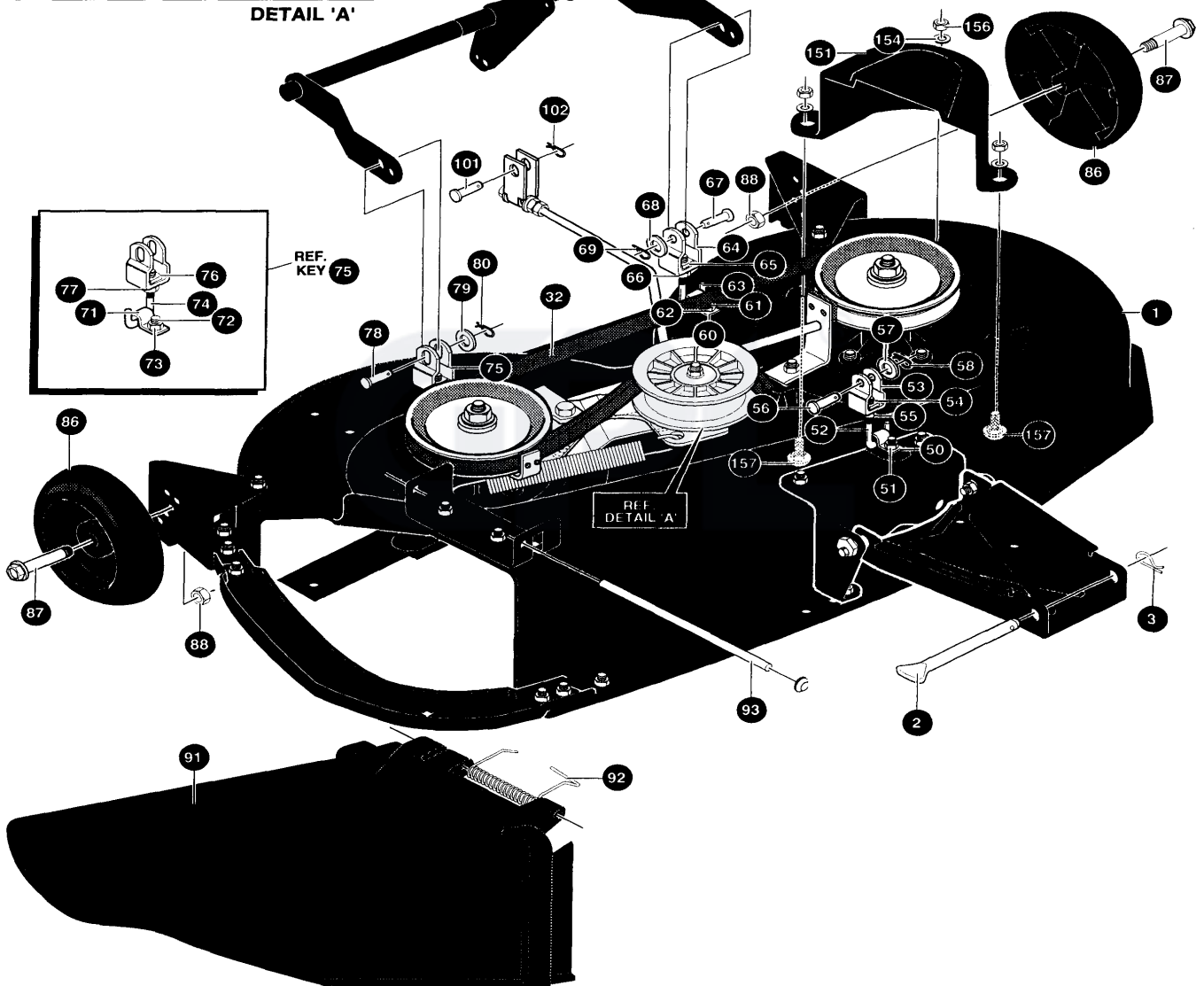
DETAIL 'A'
