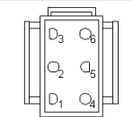
CHASSIS HARNESS CONNECTOR (MATING SIDE)
