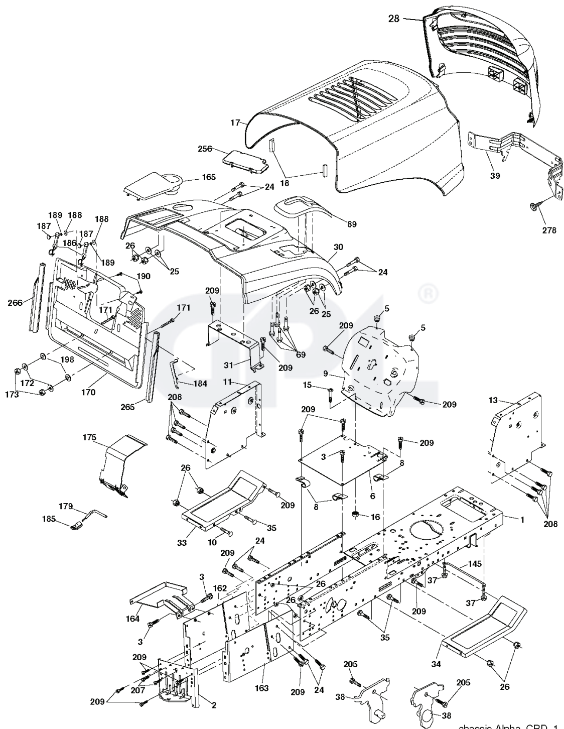
chassis-Alpha_CRD_1
