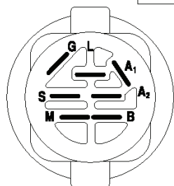
POSITION CIRCUIT "MAKE" OFF M+G+A1 RUN/OVERRIDE B+A1 RUN B+A1 L+A2 START B + S + A1
