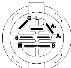
IGNITION SWITCH
