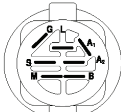
IGNITION SWITCH
