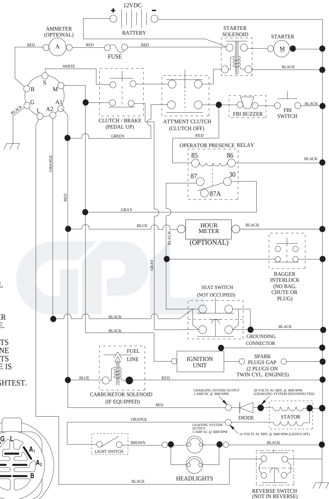
IGNITION SWITCH
