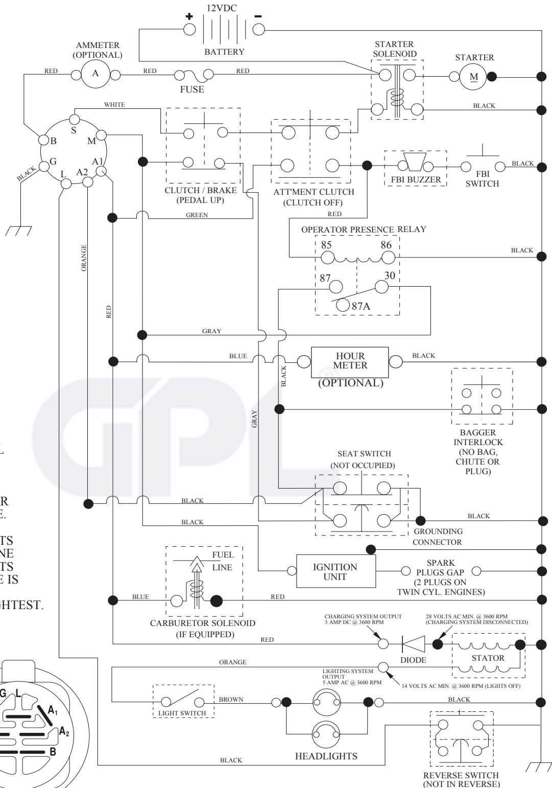
IGNITION SWITCH
