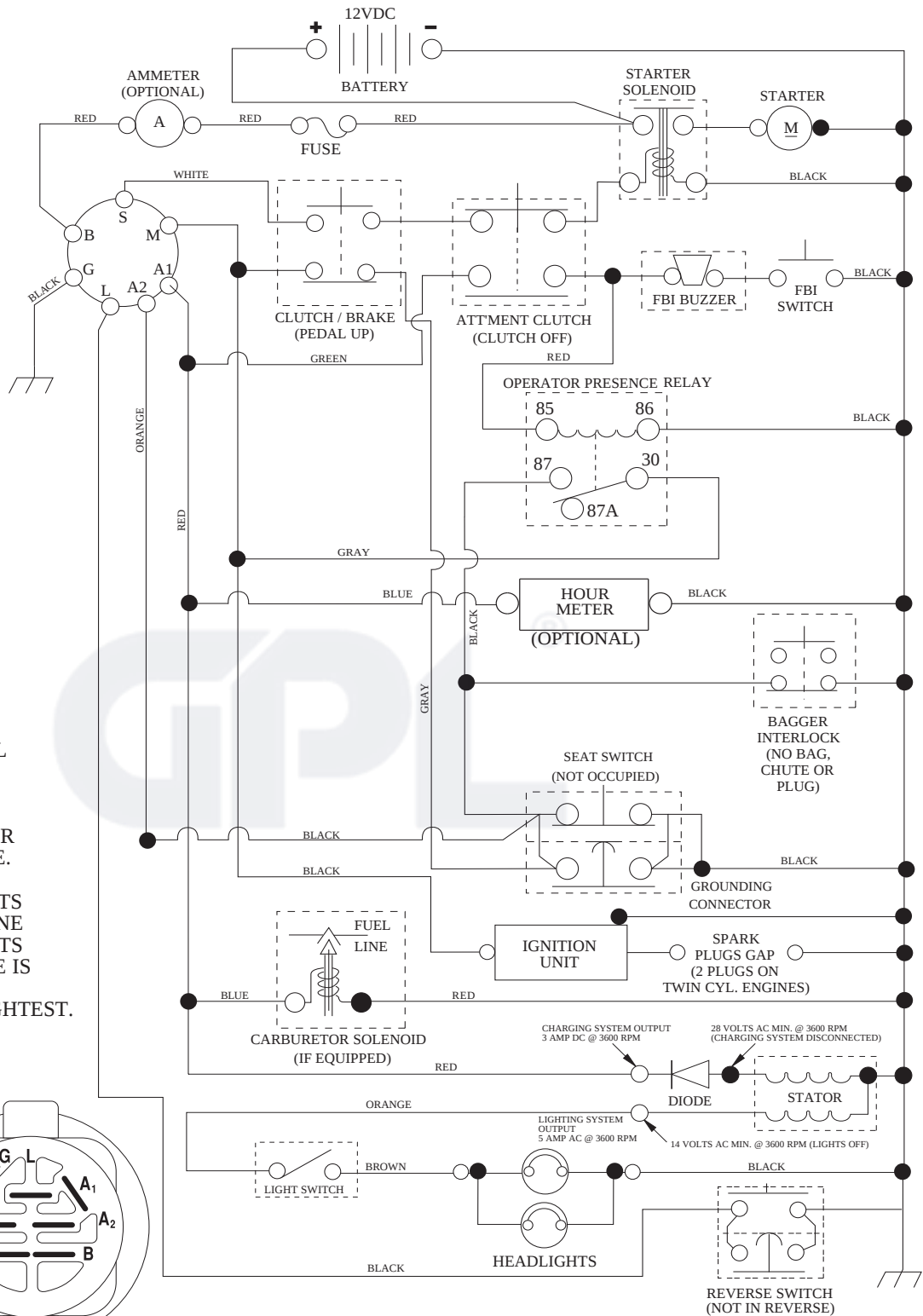
IGNITION SWITCH
