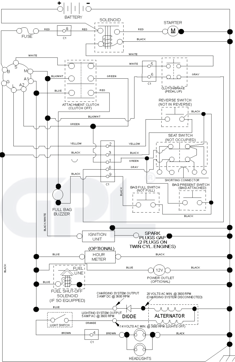
NON-REMOVABLE CONNECTIONS
