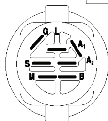
IGNITION SWITCH
