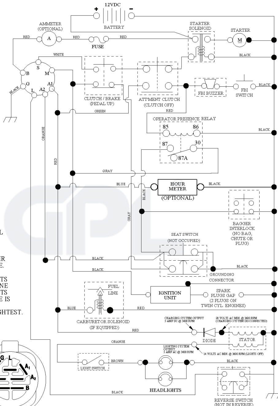
IGNITION SWITCH
