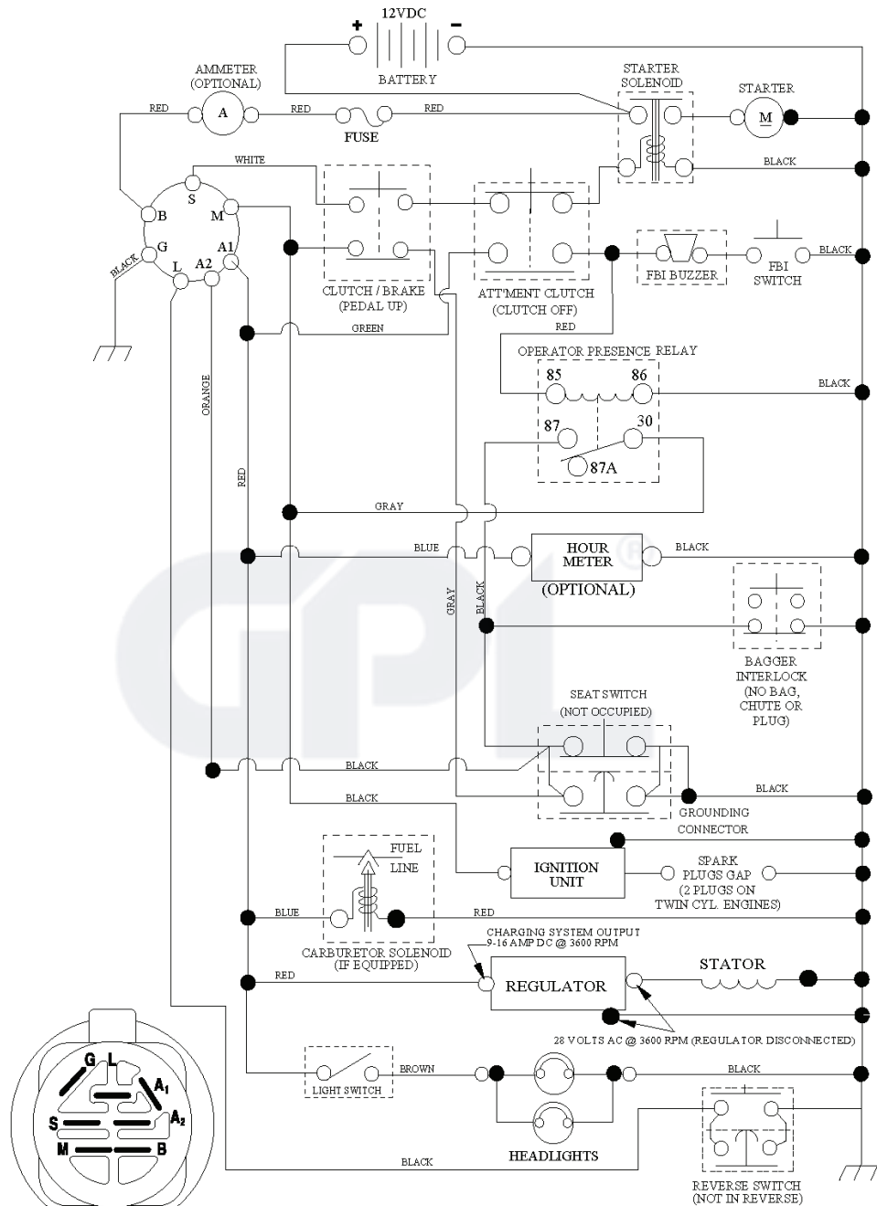
IGNITION SWITCH
