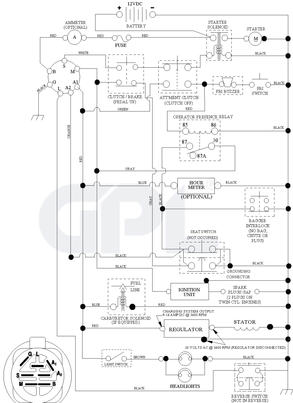
IGNITION SWITCH
