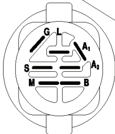
IGNITION SWITCH
