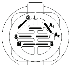
IGNITION SWITCH
