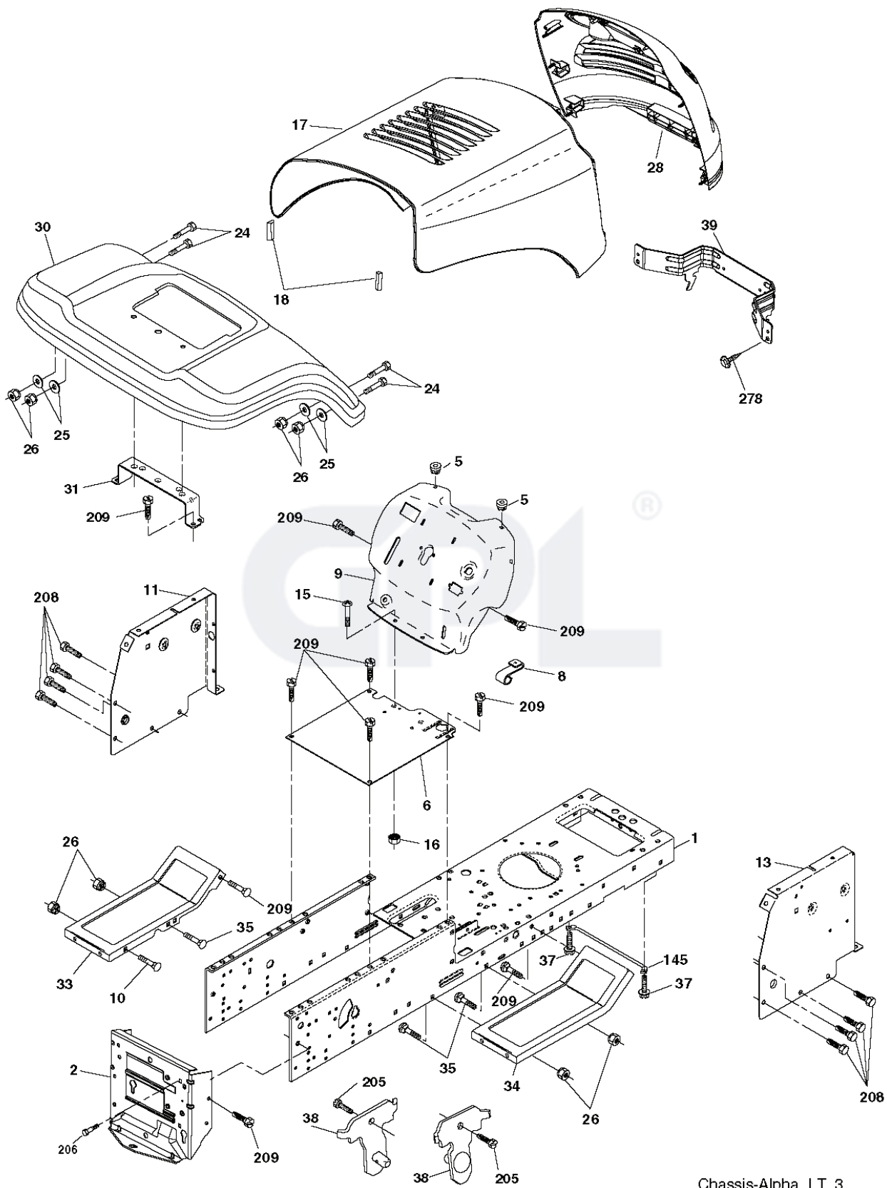
Chassis-Alpha_LT_3
