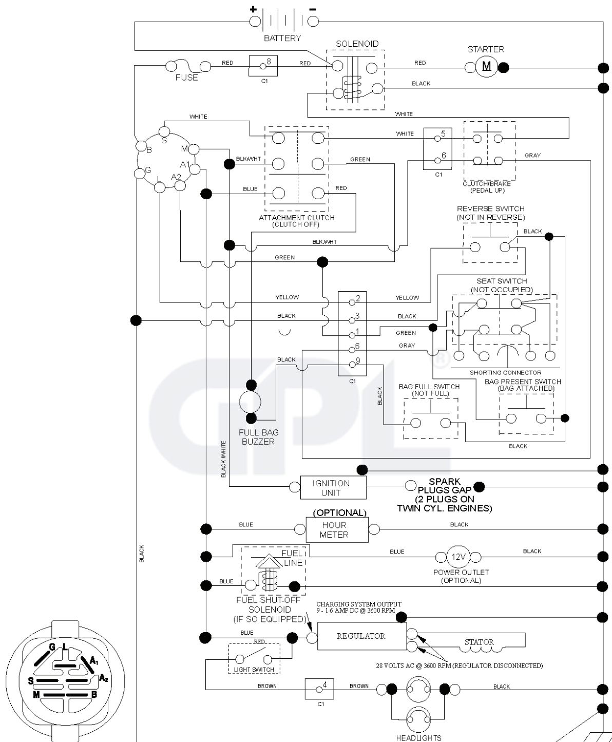
IGNITION SWITCH
