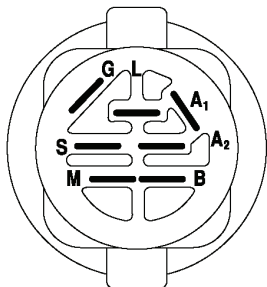
POSITION CIRCUIT "MAKE" OFF M+G+A1 NONE RUN/LIGHT B+A1 A2+L RUN B+A1 NONE START B + S + A1 NONE
