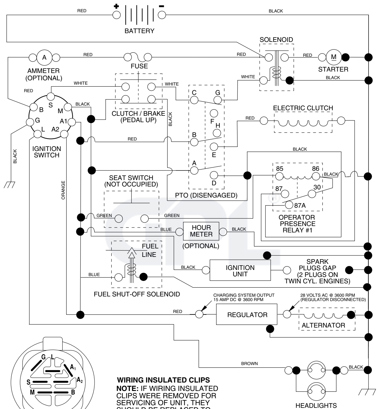
IGNITION SWITCH
