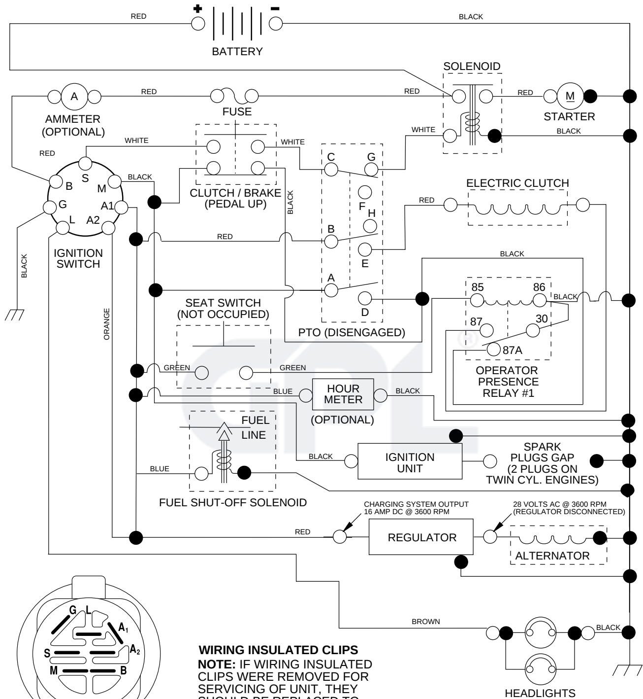
IGNITION SWITCH
