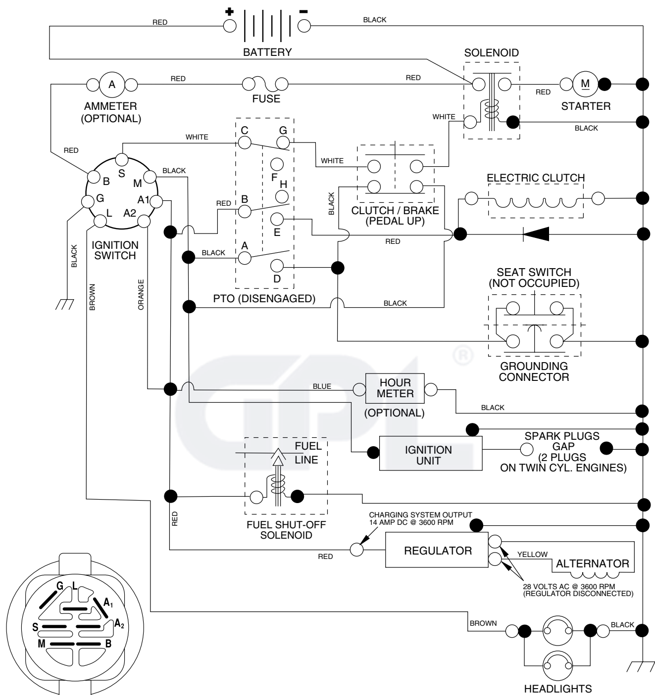
IGNITION SWITCH
