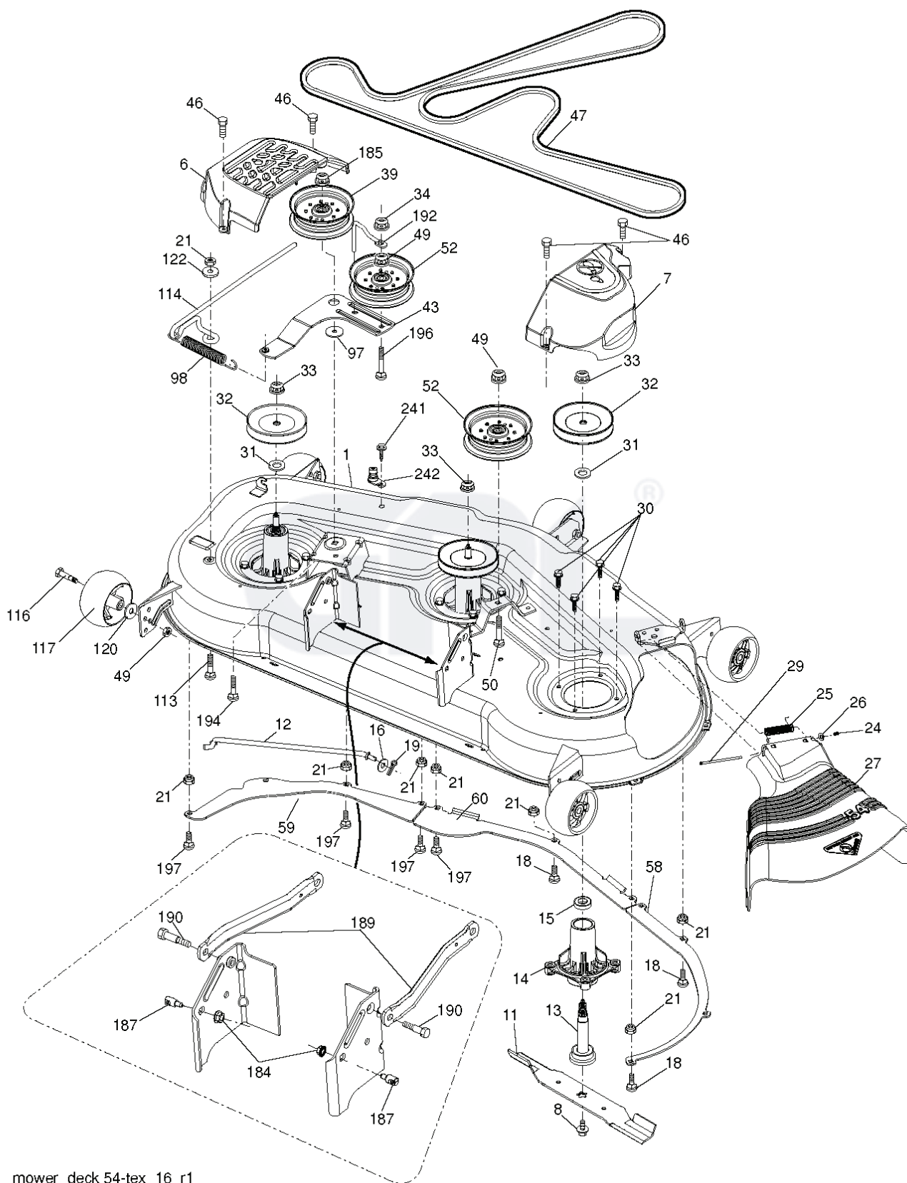
mower_deck 54-tex_16_r1
